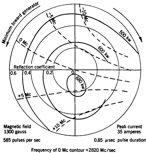
FIG. 19-27.—Rieke diagram for HP10V magnetron.
